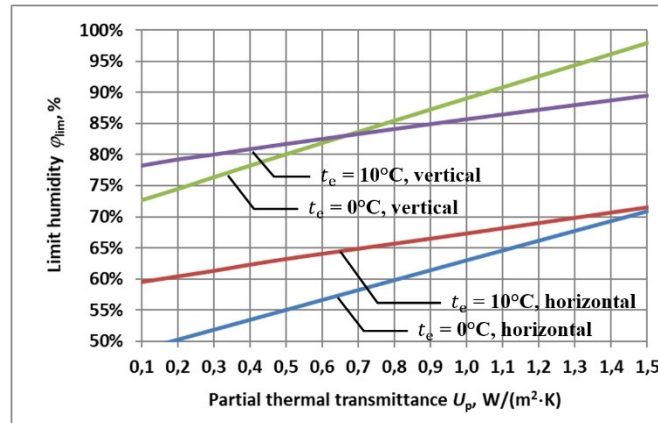
Fig. 2. Dependence of air humidity, at which water vapor condensation on the envelope surface is possible, on its insulation, for \varepsilon = 0.85 (own research)
