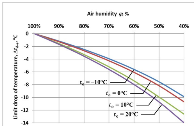
Fig. 1. Temperature drop necessary to reach the dew point on the surface, description in the text (own research)
