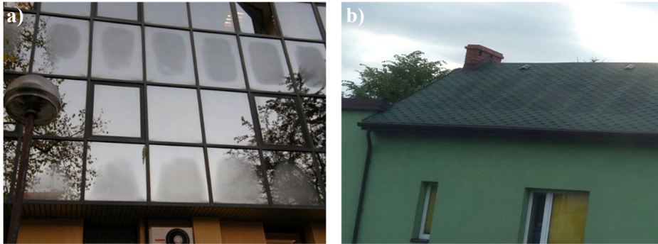
Fig. 3. Typical forms of external condensation of water vapor on envelopes: a) on the glass facade; no condensation in the upper part of the room and near poorly insulated structural frames, b) on the roof slope; no condensation in places of poorly insulated rafters ( own photos )
