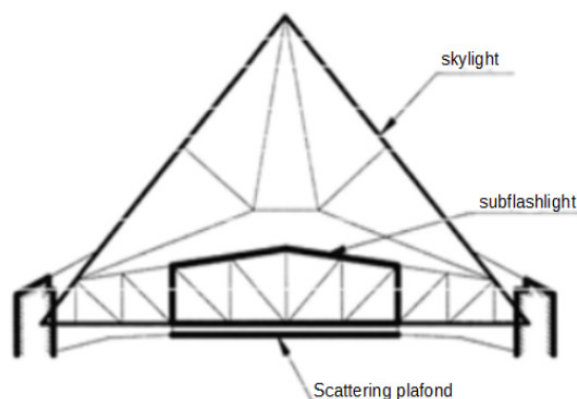
Fig. 3. Diagram of fenestration of the Pushkin Museum of Fine Arts ( own study )
