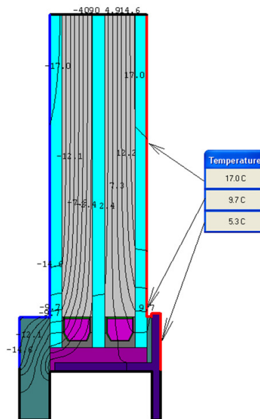
Fig. 5. Temperature distribution over the inner surface of the glazing of the subflashlight when using a IGU 4И-10Kr-4-10Kr-4И ( own study )
