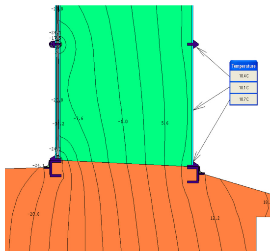
Fig. 4. Temperature distribution over the inner surface of the lower part of the fenestration, manufactured according to Option 5, with t_{\text{H}} = -28^{\circ}\text{C} ( own study )
